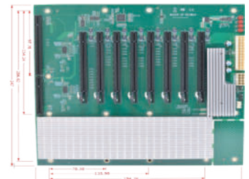
PicMG Backplane
